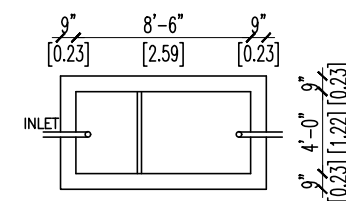
DETAILS OF SEPTIC TANK
