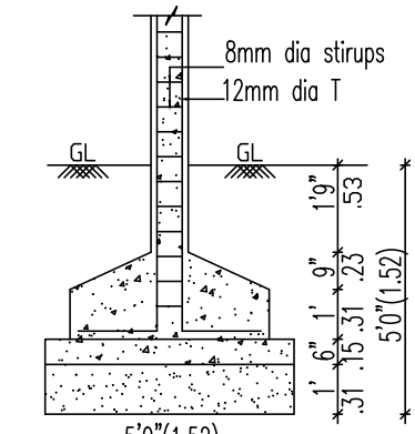
COLUMN FOUNDATION DETAIL SCALE 1":4'0"(1:50)
