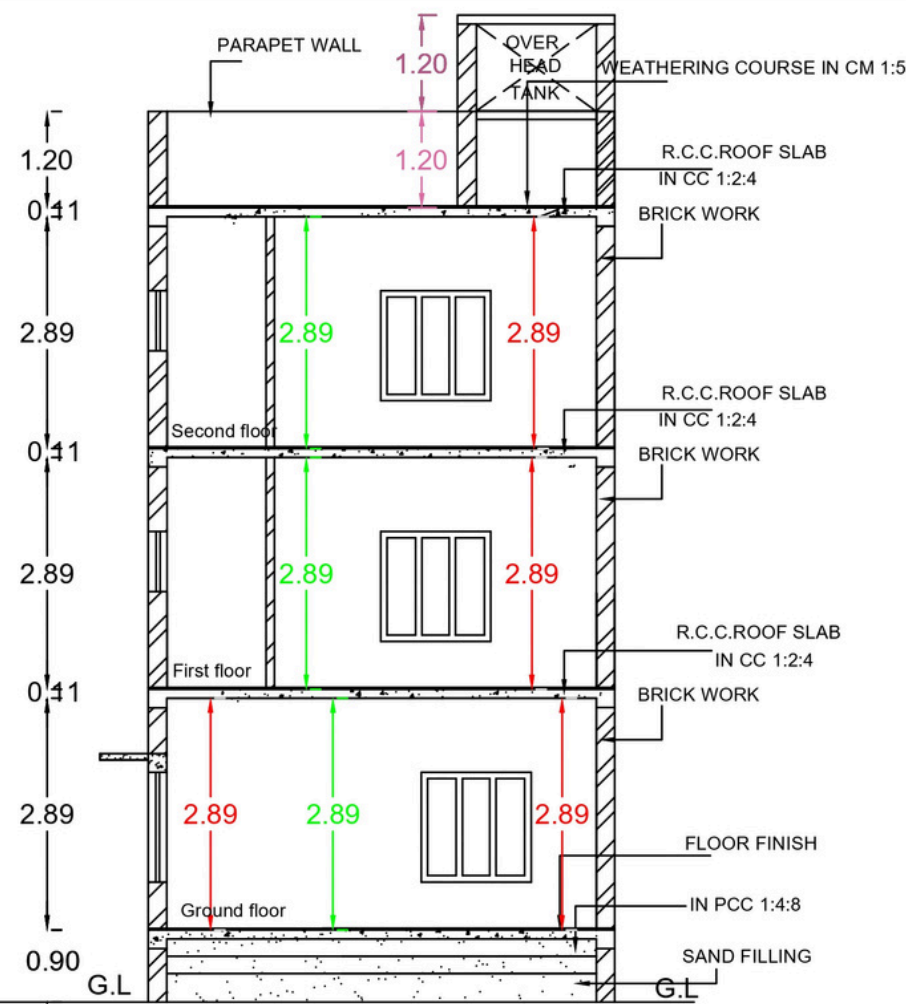
SECTION "AA"
