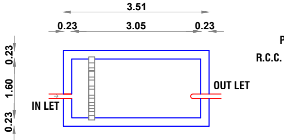
PLAN OF SEPTIC TANK CAPACITY - 8000 LITRES
