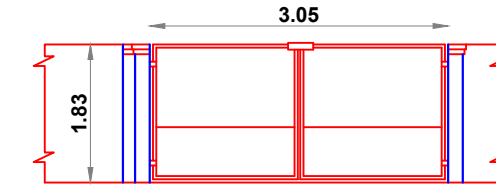
ELEVATION OF COMPOUND WALL
