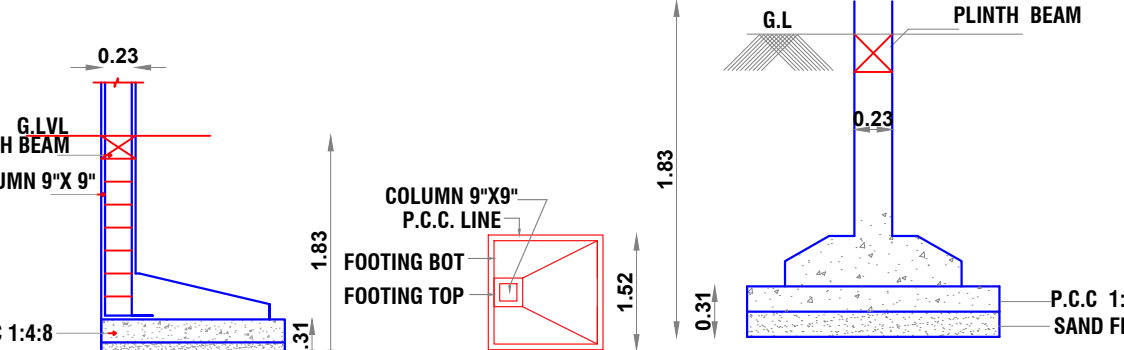
END FOOTING DETAILS
