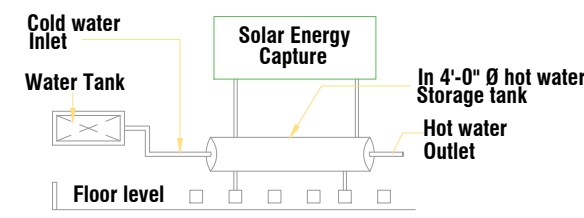
SOLAR HOT WATER SYSTEM DETAIL
