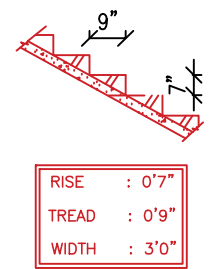
STAIRS DETAILS
