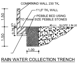
RAIN WATER COLLECTION TRENCH
