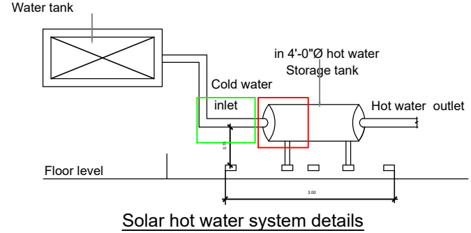
Solar hot water system details
