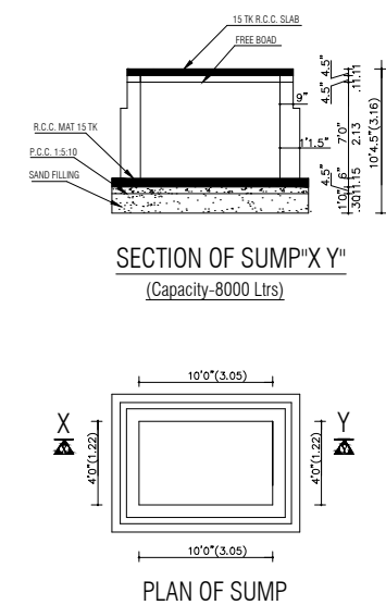
PLAN OF SUMP
