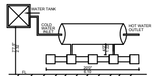
SOLAR HOT WATER SYSTEM DETAILS
