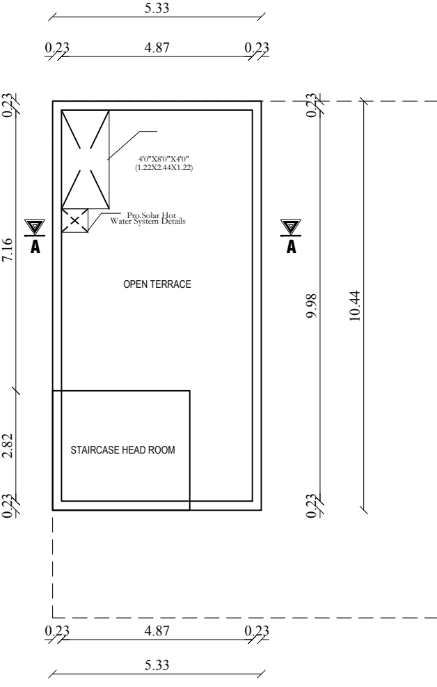
PRO.TERRACE FLOOR PLAN
