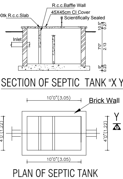
PLAN OF SEPTIC TANK
