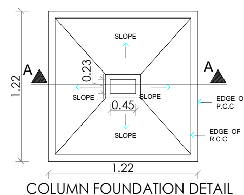
COLUMN FOUNDATION DETAIL
