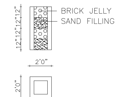
PERCULATION PIT
