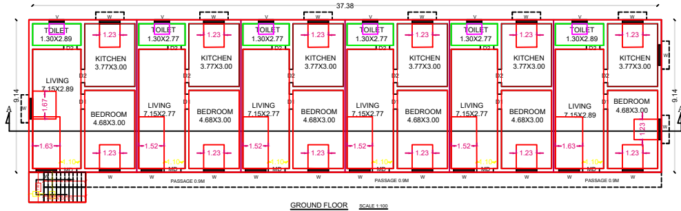
GROUND FLOOR SCALE 1:100
