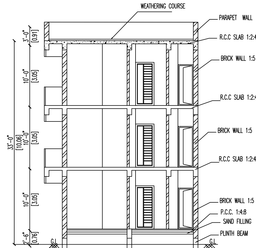
SECTION -AA
