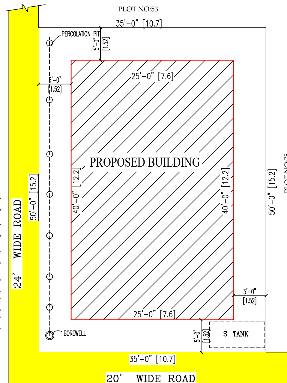
SITE PLAN
