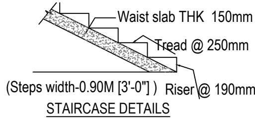
STAIRCASE DETAILS
