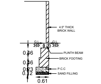
COMPOUND WALL
