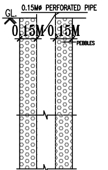
PLAN BORE WELL "nts"
