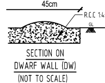
SECTION ON DWARF WALL (DW) (NOT TO SCALE)
