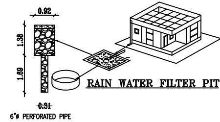
RAIN WATER FILTER PIT
