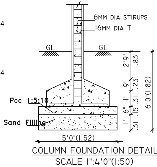
COLUMN FOUNDATION DETAIL SCALE 1"=4'0" (1:50)
