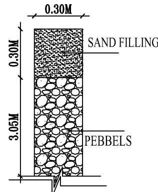
PERCOLATION PIT
