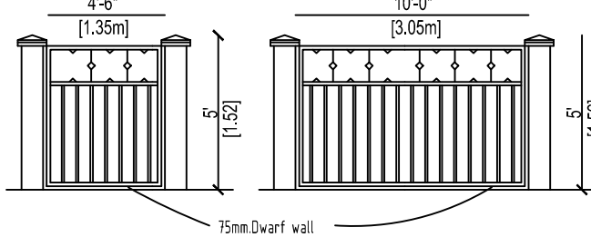
GATE ELEVATION (NTS)
