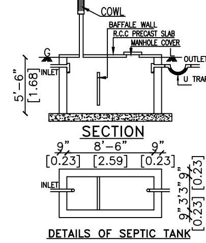
DETAILS OF SEPTIC TANK
