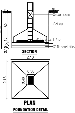
FOUNDATION DETAIL
