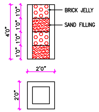
PERCOLATION PIT
