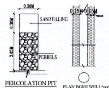
PERCOLATION PIT PLAN BORE WELL
