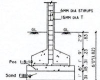
COLUMN FOUNDATION DETAIL SCALE 1"=4'-0" (1:50)
