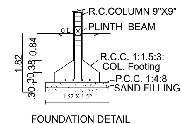
FOUNDATION DETAIL
