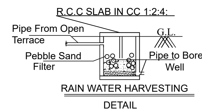
DETAIL
