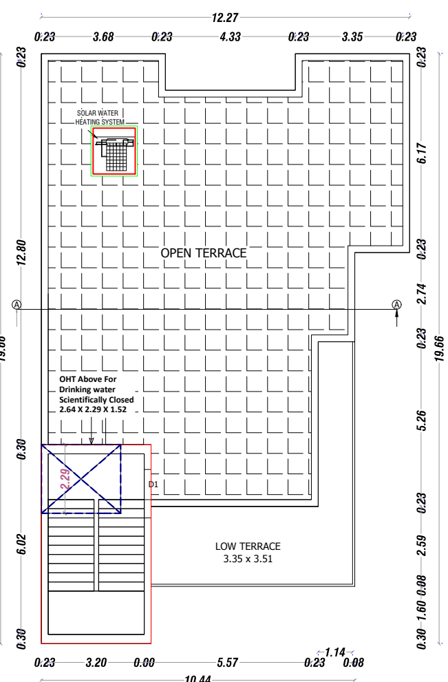
TERRACE FLOOR PLAN (PROPOSED)
