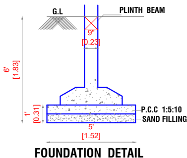
FOUNDATION DETAIL
