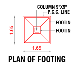
PLAN OF FOOTING
