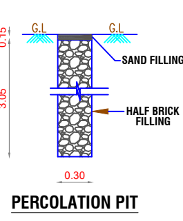
PERCOLATION PIT
