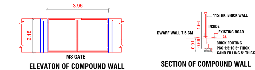
ELEVATION OF COMPOUND WALL
