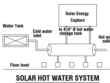
SOLAR HOT WATER SYSTEM
