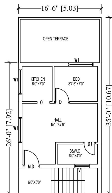
PROPOSED SECOND FLOOR PLAN
