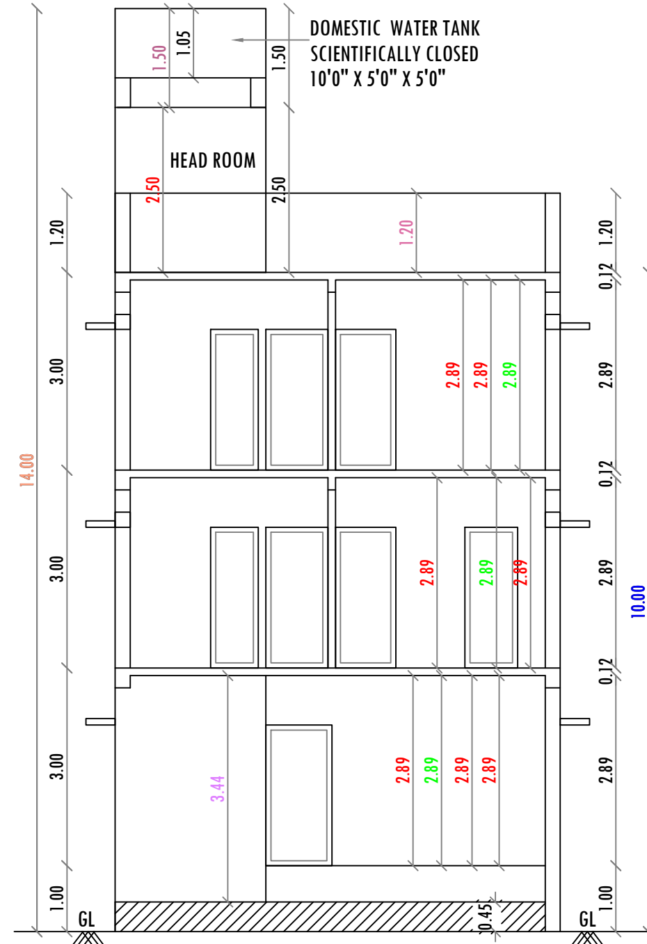
SECTION ON 'A-A' (PROPOSED)
