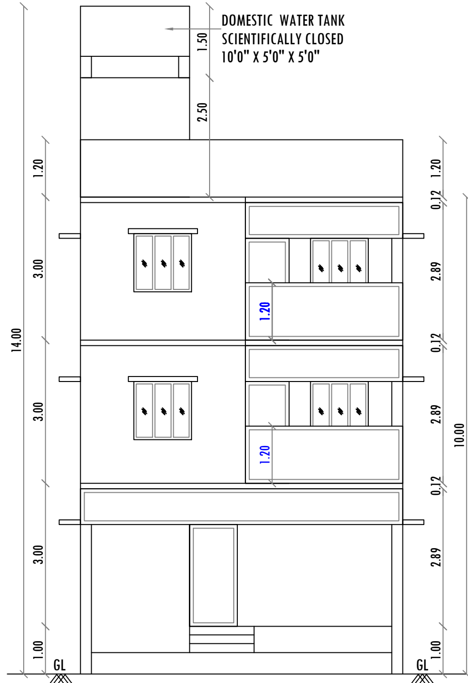
ELEVATION (PROPOSED)
