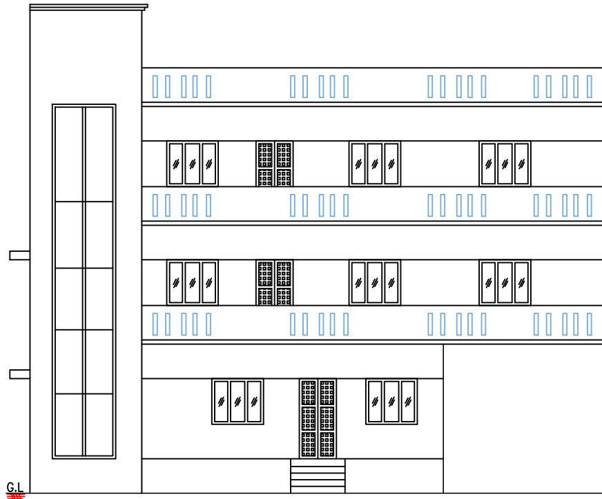
FRONT ELEVATION
