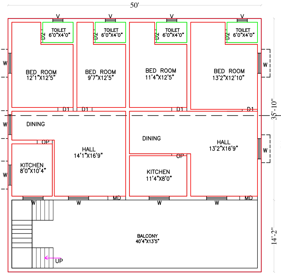
TYPICAL FIRST & SECOND FLOOR PLAN TYPICAL_FLOOR_PLAN=1,2
