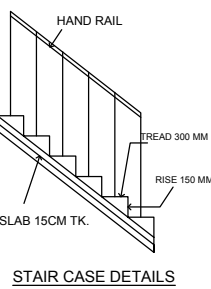
STAIR CASE DETAILS
