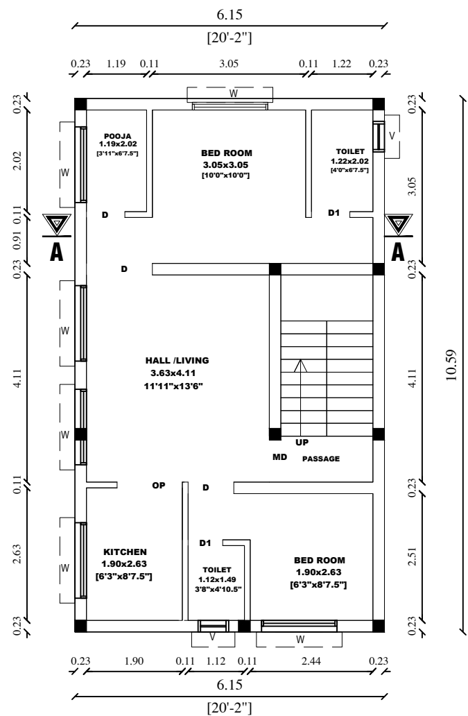
PRO.FIRST FLOOR
