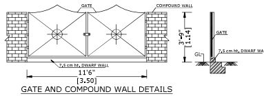
GATE AND COMPOUND WALL DETAILS
