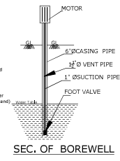
SEC. OF BOREWELL
