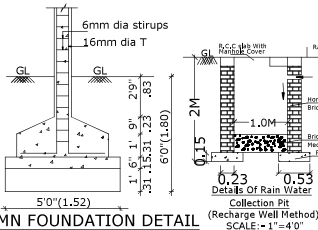
COLUMN FOUNDATION DETAIL
