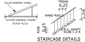
STAIRCASE DETAILS
