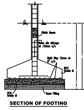
SECTION OF FOOTING
