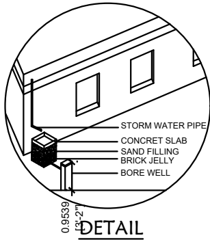
RAINWATER HARVESTING
