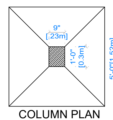
TYPICAL FOUNDATION DETAIL
