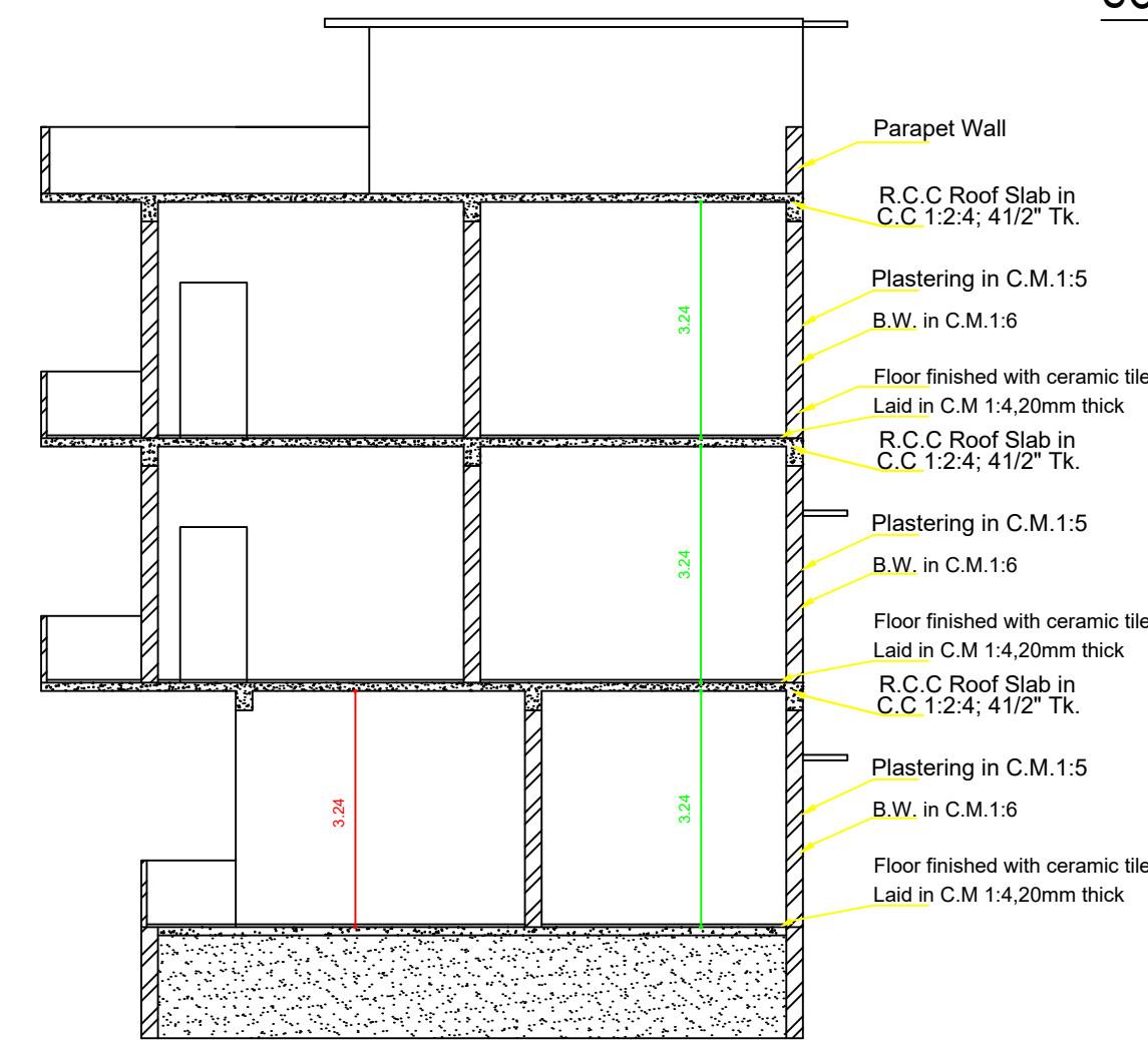
SECTION
