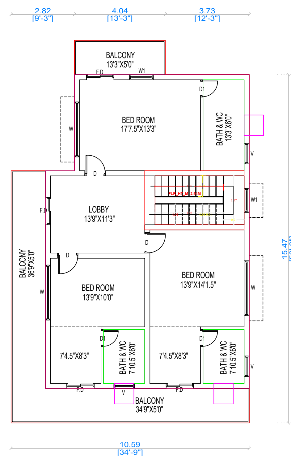
TYPICAL I & II-nd FLOOR PLAN
