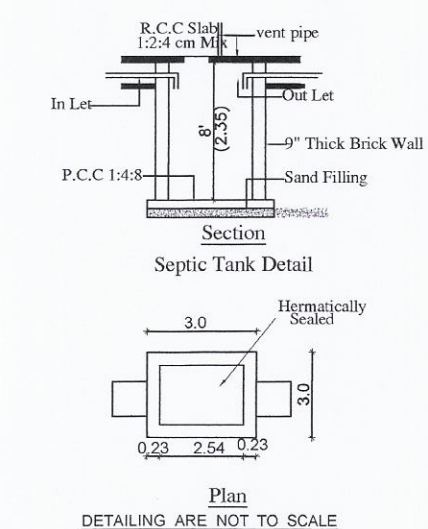
DETAILING ARE NOT TO SCALE
