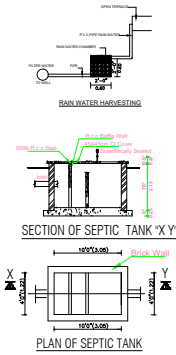
PLAN OF SEPTIC TANK
