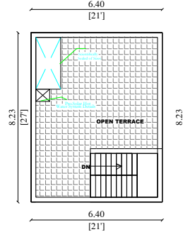
PROPOSED TERRACE FLOOR PLAN
