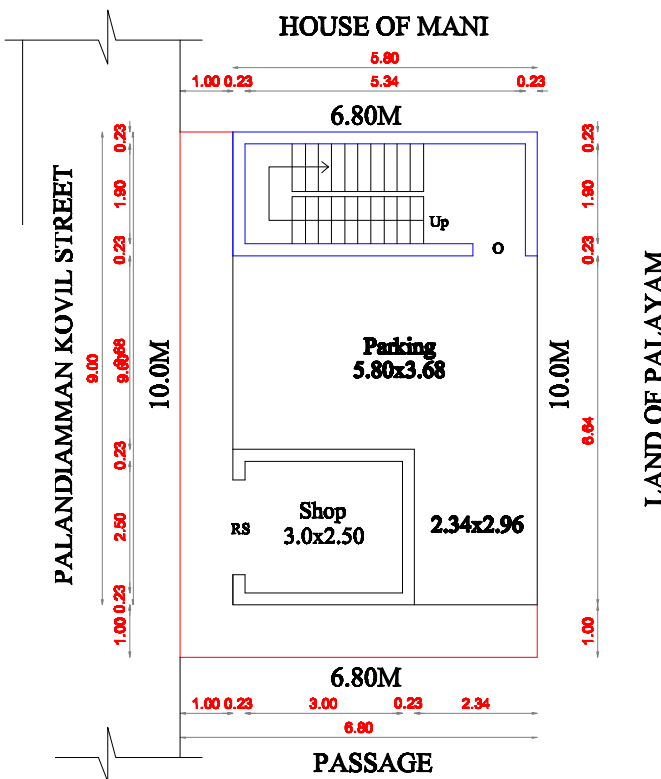
PRO.SITE CUM GROUND FLOOR PLAN
