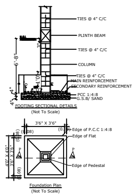
FOUNDATION PLAN
