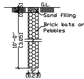
Percolation Pit
