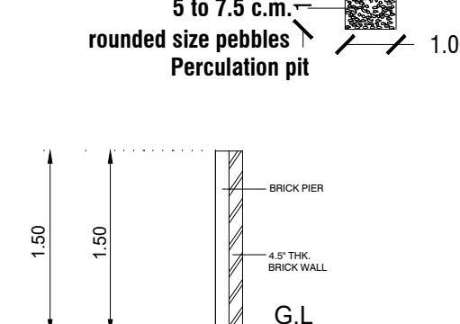
COMPOUND WALL DETAIL
