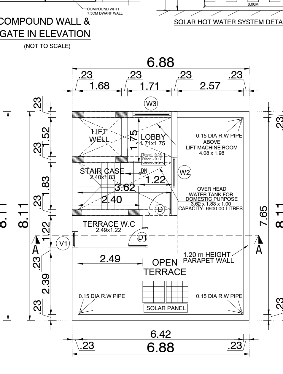
TERRACE FLOOR PLAN (PROPOSED)
