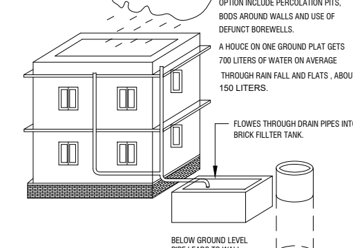
Rain Water Storage Details
