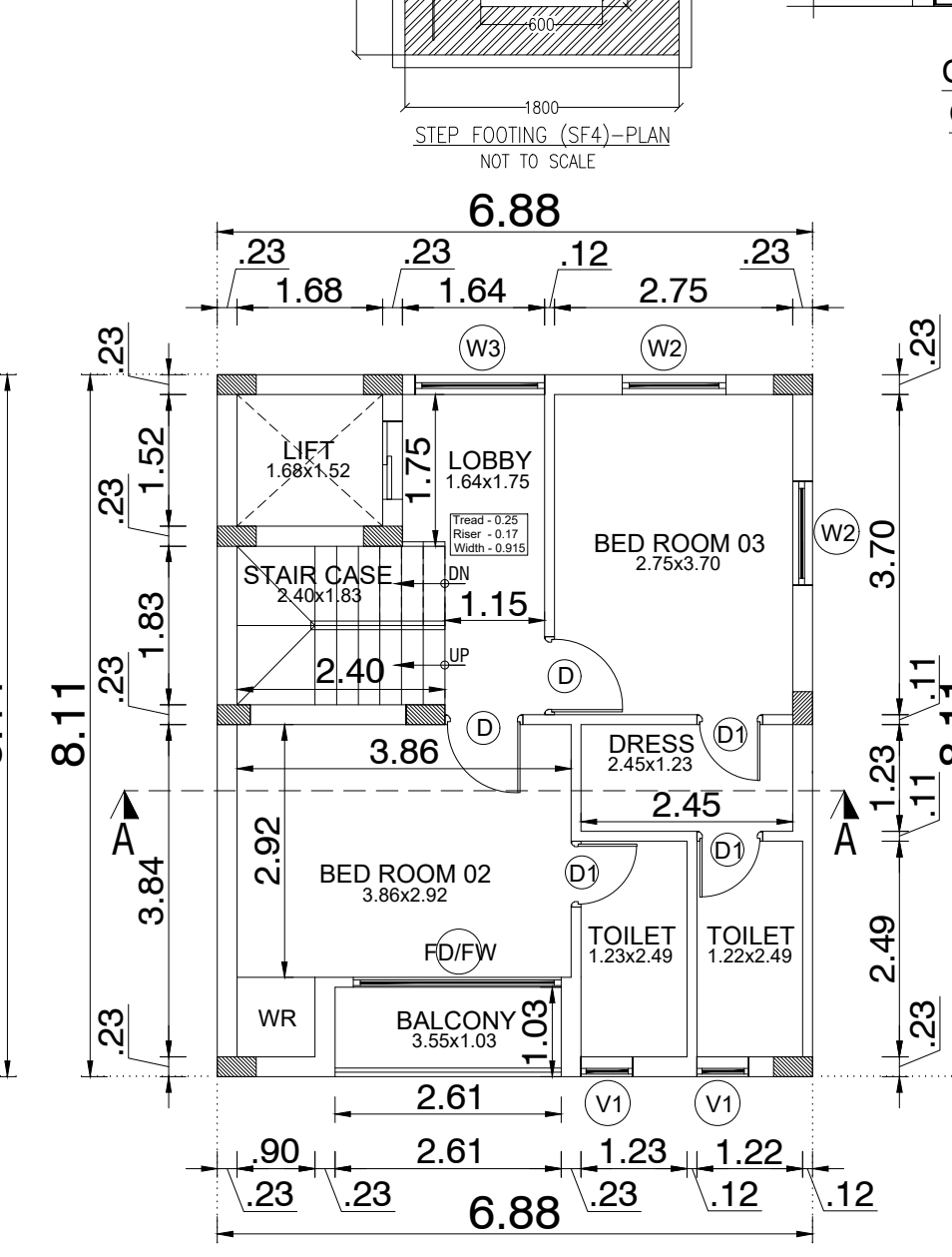
SECOND FLOOR PLAN (PROPOSED)
