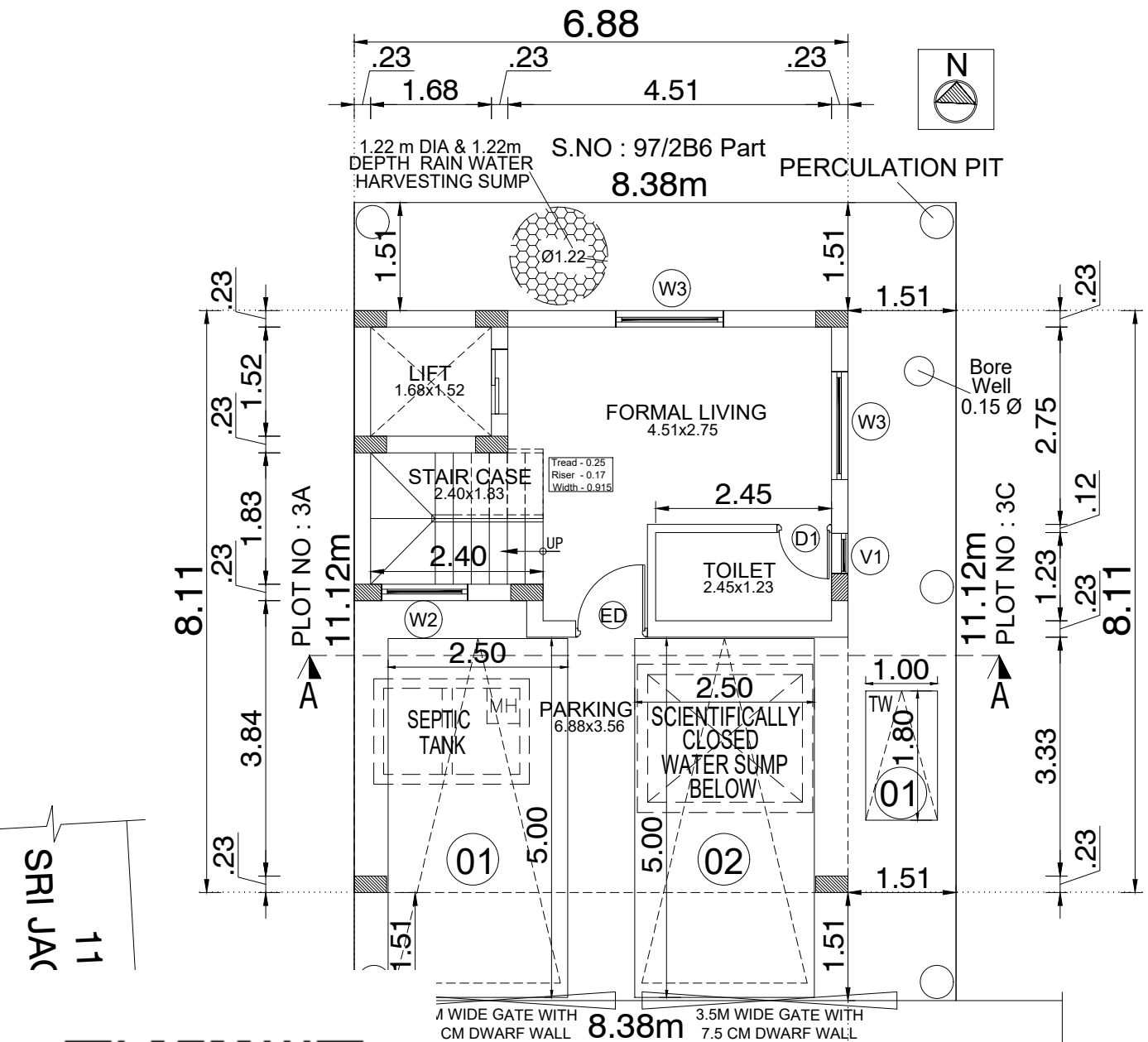
CUM GROUND FLOOR PLAN (PART)
