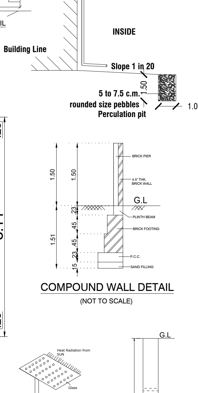
DWARF WALL DETAILS
