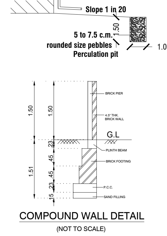
COMPOUND WALL DETAIL (NOT TO SCALE)
