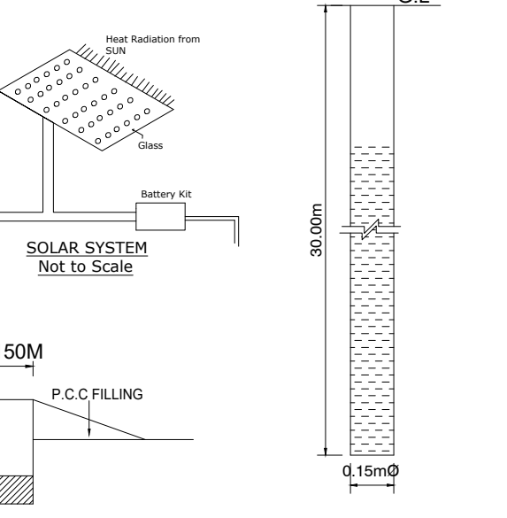
Bore Well Details Scale 1:1.5
