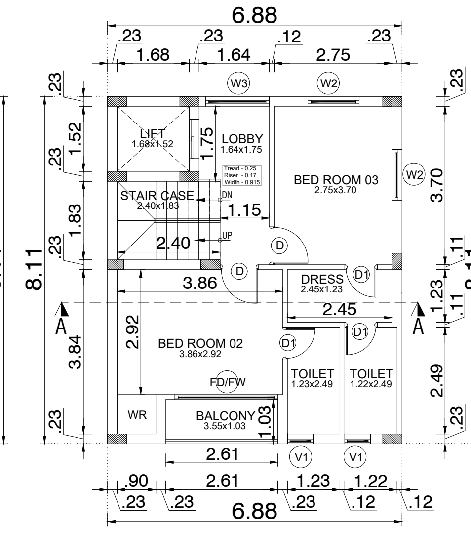
SECOND FLOOR PLAN (PROPOSED)
