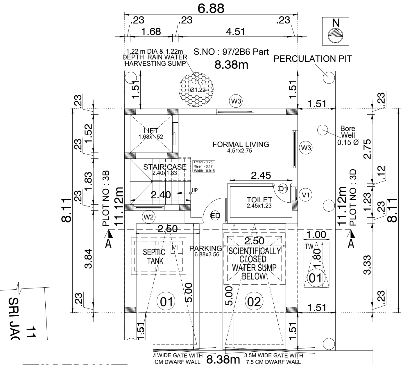
CUM GROUND FLOOR PLAN (PART) (PROPOSED)
