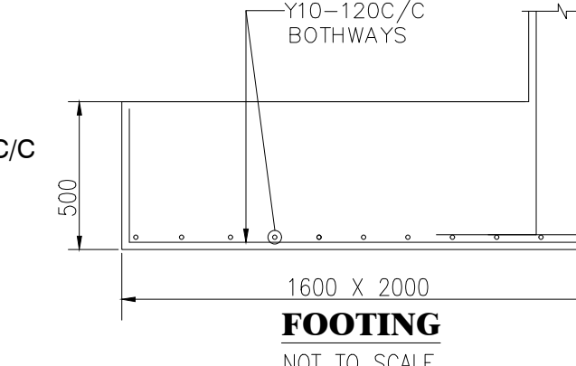
FOOTING NOT TO SCALE
