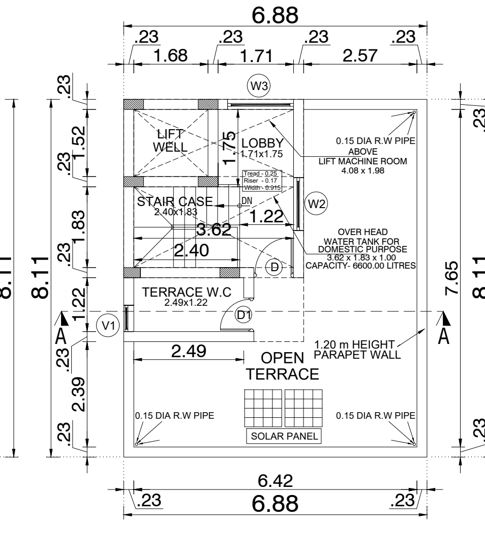
TERRACE FLOOR PLAN (PROPOSED)
