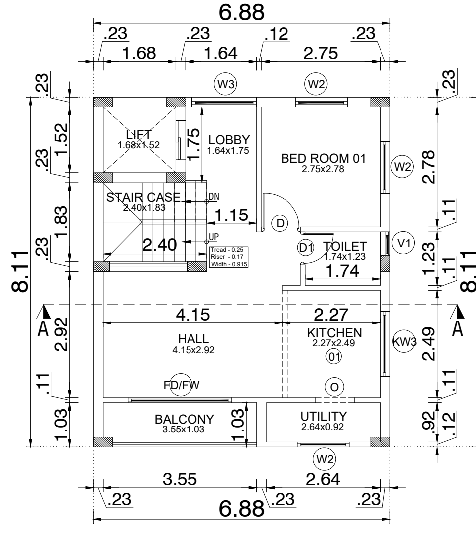
FIRST FLOOR PLAN (PROPOSED)
