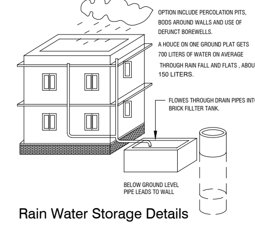
Rain Water Storage Details
