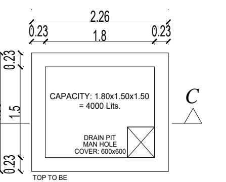
PLAN OF SUMP (NOT TO SCALE)
