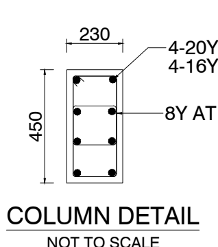
COLUMN DETAIL NOT TO SCALE
