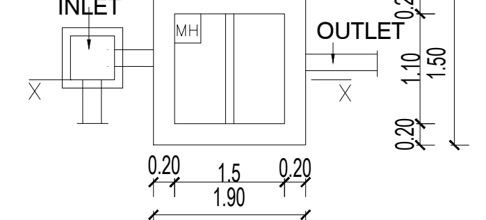
PLAN OF SUMP (NOT TO SCALE)
