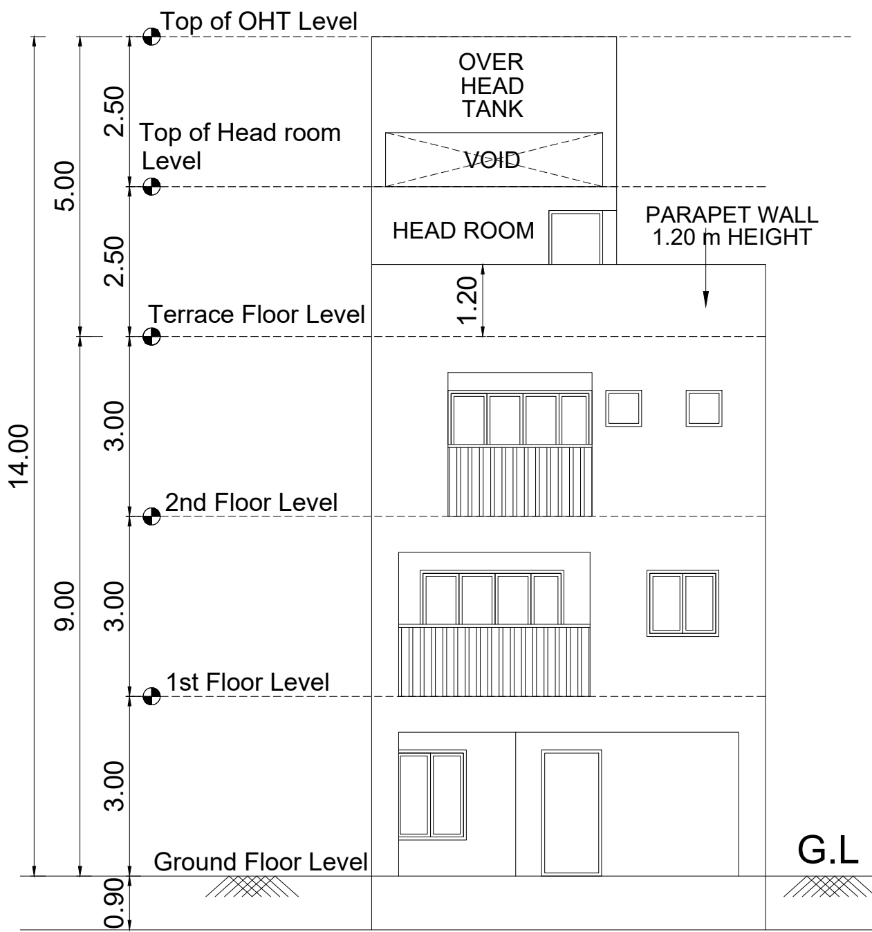
SOUTH SIDE ELEVATION
