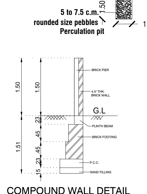
COMPOUND WALL DETAIL (NOT TO SCALE)
