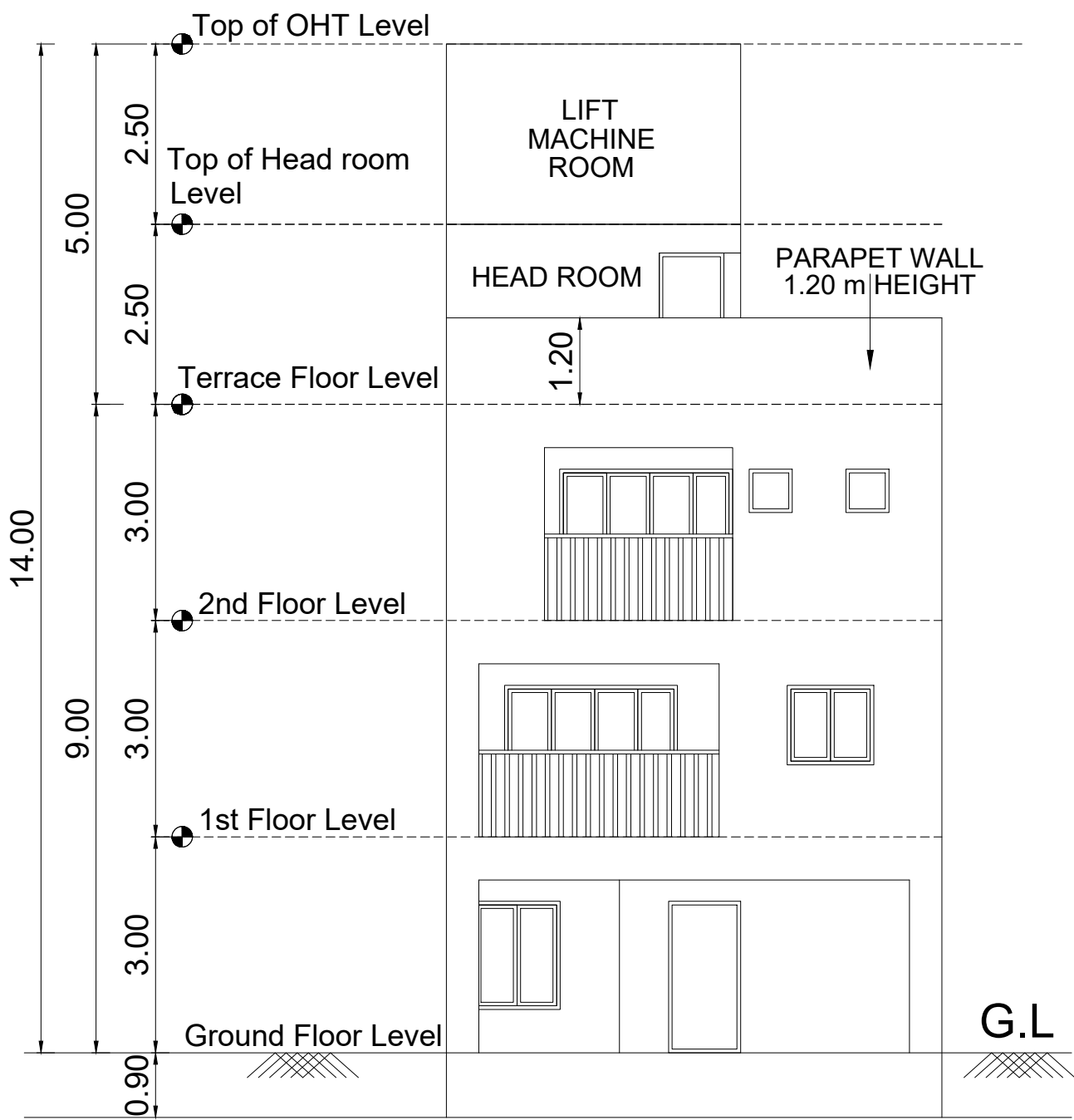
NORTH SIDE ELEVATION
