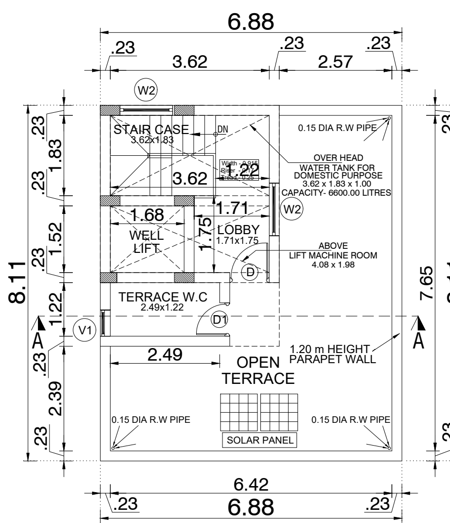
TERRACE FLOOR PLAN (PROPOSED)
