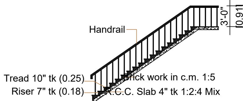
Staircase Details
