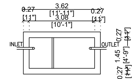
PLAN DETAILS OF SEPTIC TANK
