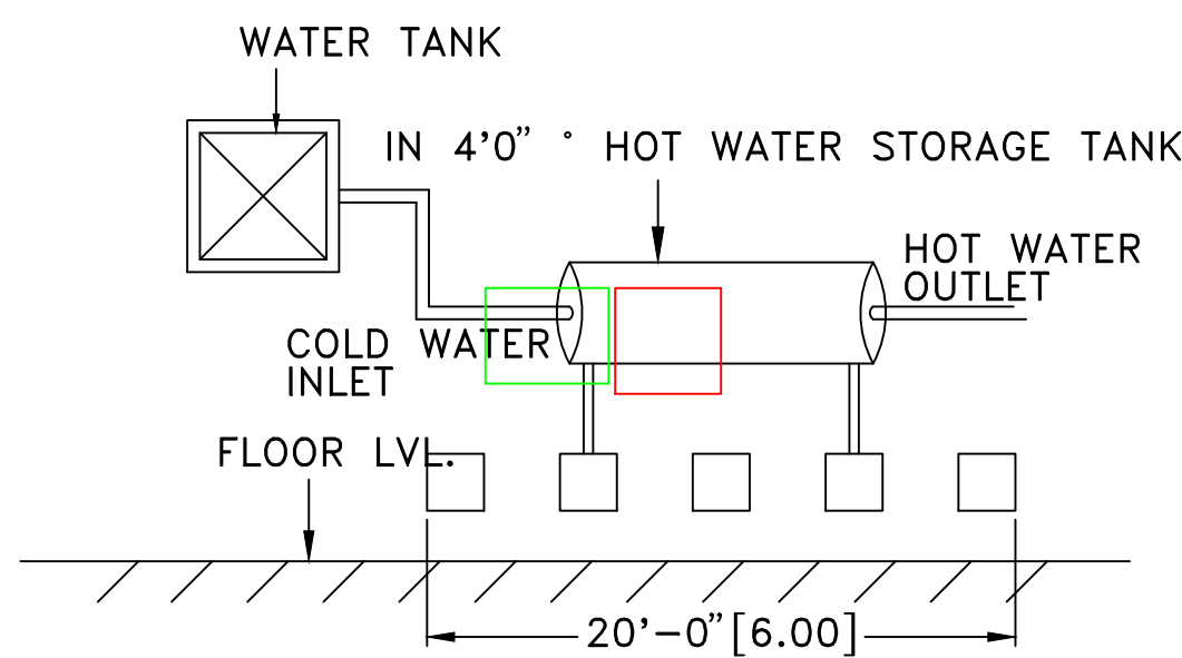
SOLAR HOT WATER SYSTEM DETAIL
