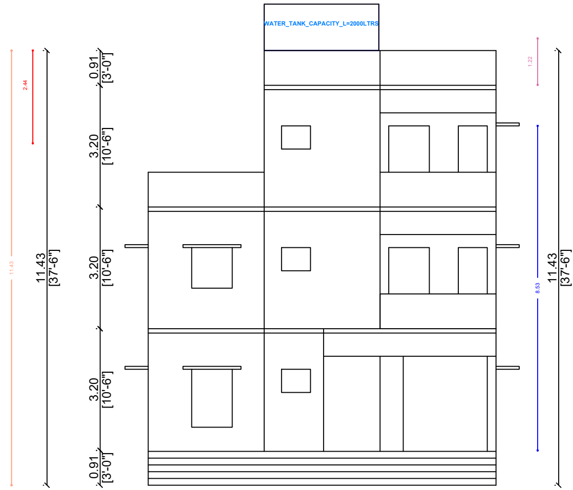
FRONT ELEVATION
