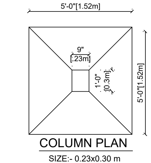
TYPICAL FOUNDATION DETAIL Footing Detail
