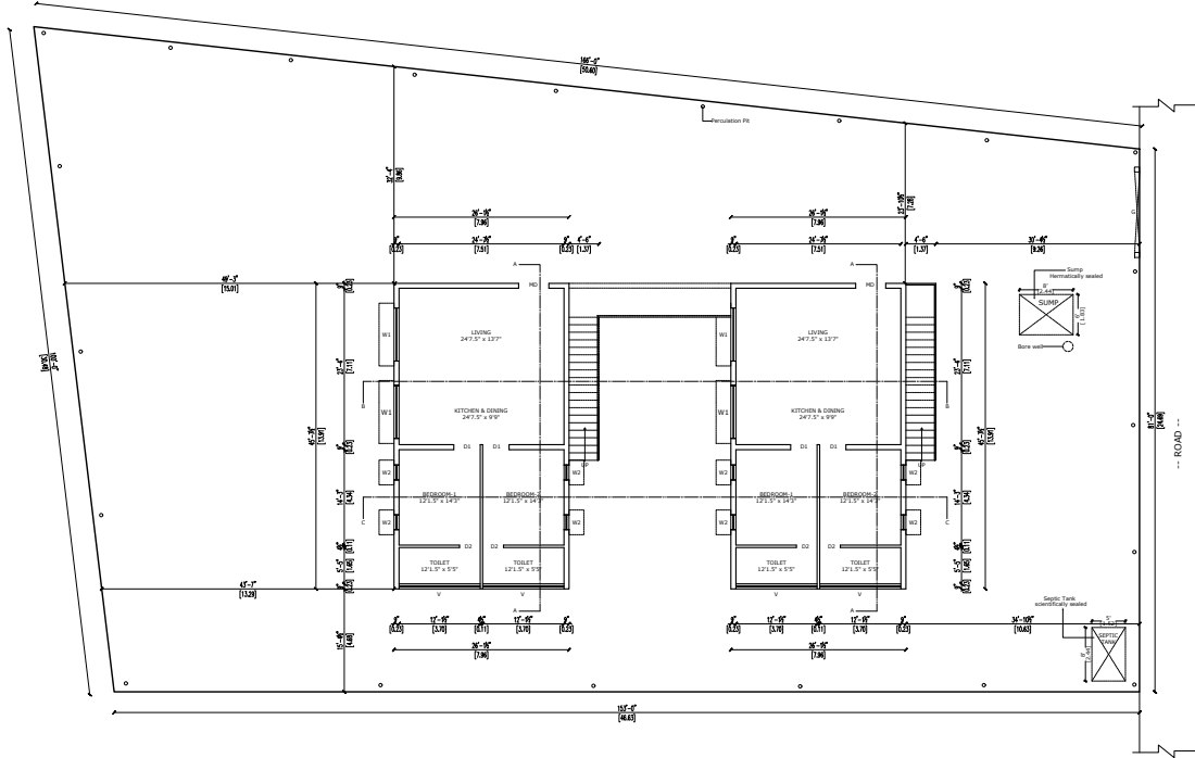
SITE/GROUND FLOOR PLAN
