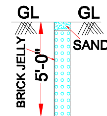
PERCOLATION PIT
