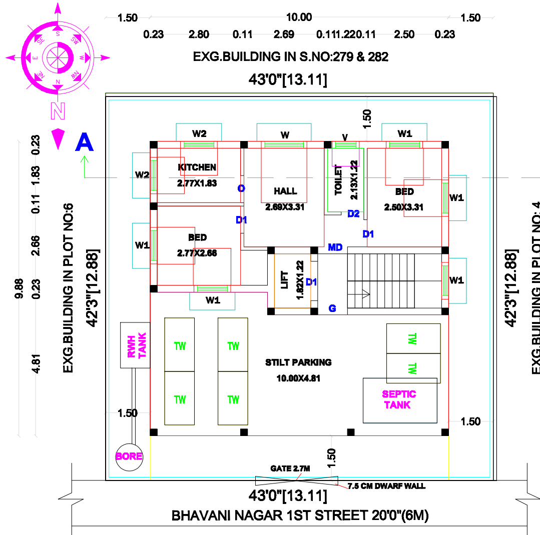
SITE/STILT CUM GROUND FLOOR PART PLAN
