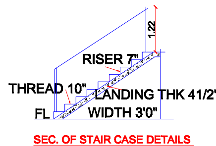
SEC. OF STAIR CASE DETAILS
