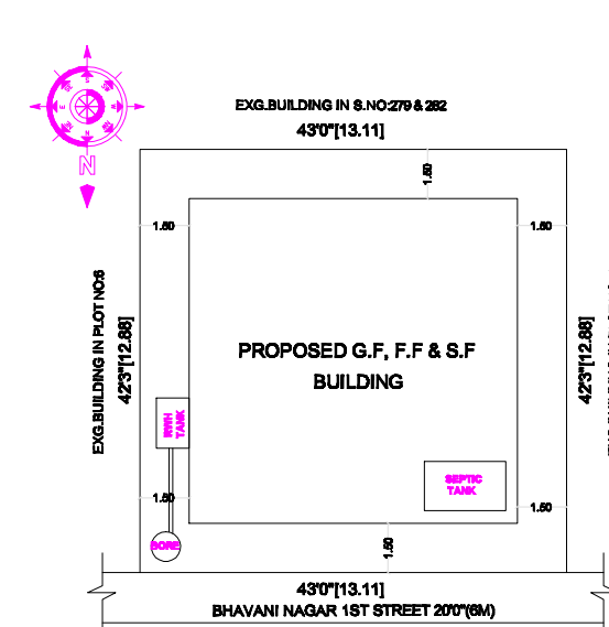
SITE & PROPOSED PLAN
