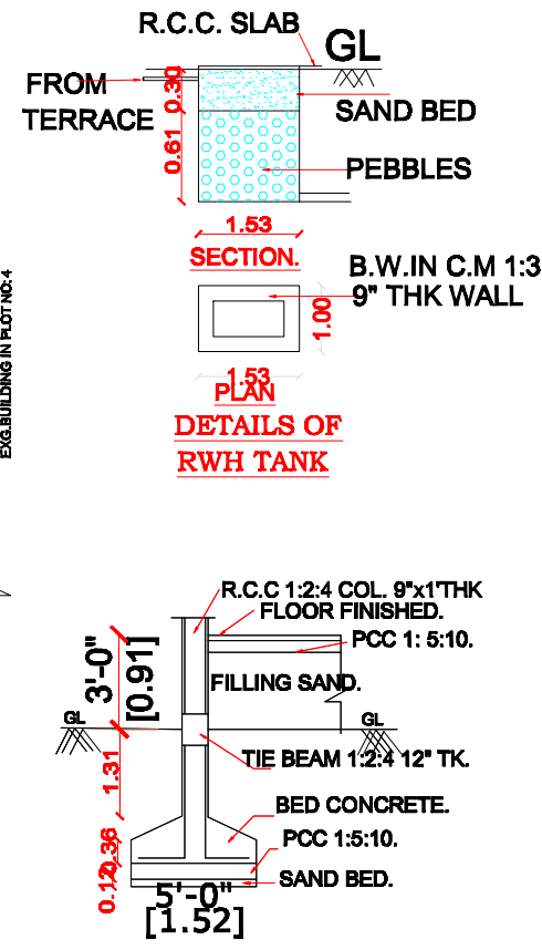
COLUMN FOUNDATION
