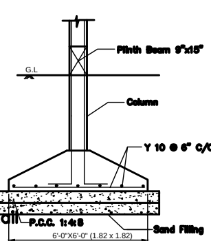
Footing Section (Scale : Nts)
