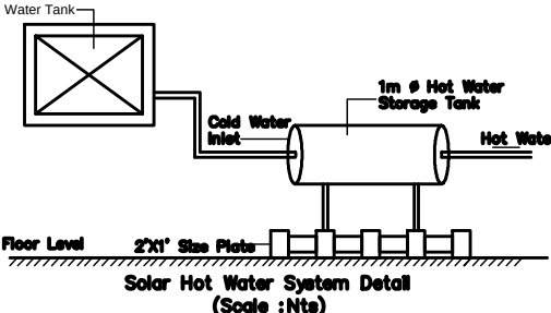
Solar Hot Water System Detail (Scale : Nts)
