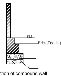
Section of compound wall (Scale : NTS)
