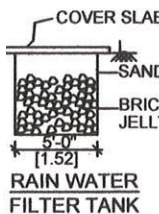
RAIN WATER FILTER TANK
