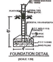
FOUNDATION DETAIL
