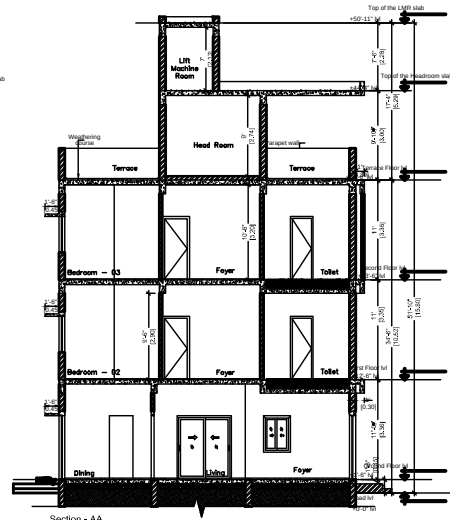
SECTION
