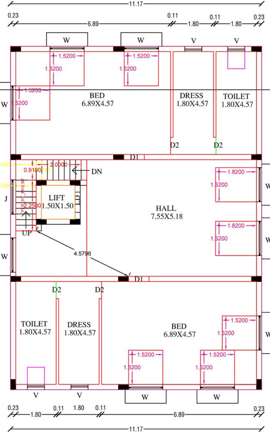
TYPICAL FLOOR PLAN SECOND AND THIRD FLOOR PLAN
