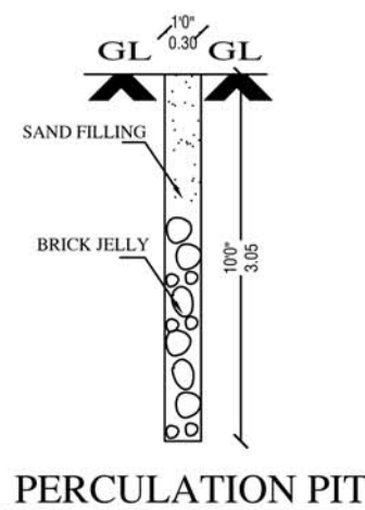
PERCOLATION PIT
