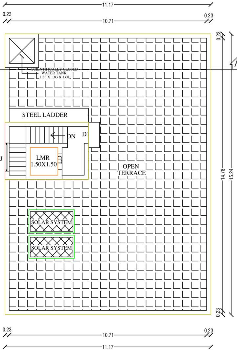
TERACE FLOOR PLAN
