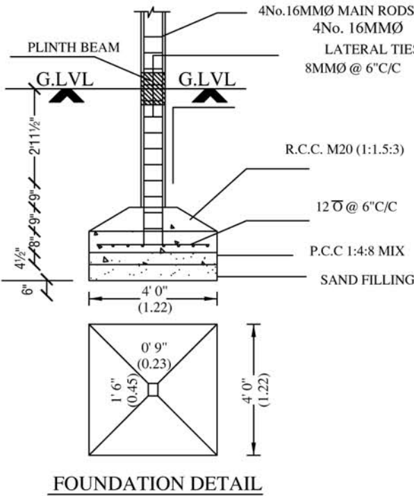
FOUNDATION DETAIL
