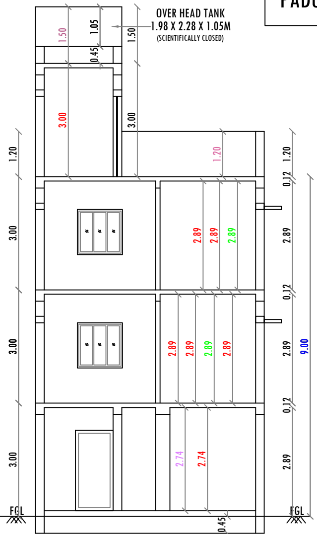
SECTION 'A-A'
