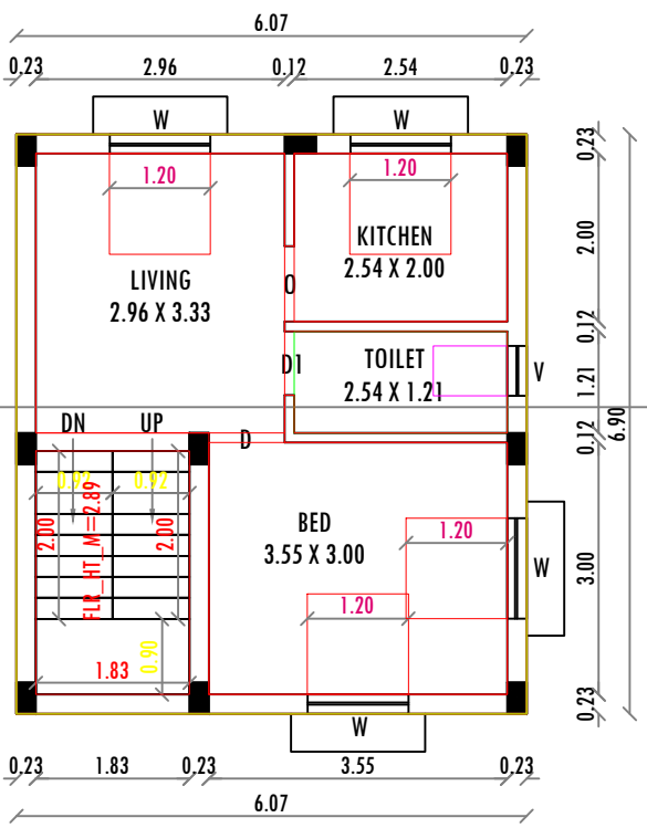
FIRST FLOOR PLAN (PROPOSED)
