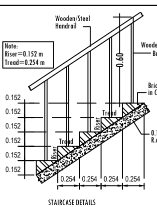
STAIRCASE DETAILS (Scale 1:25)
