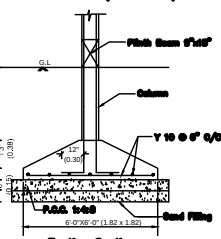
Section of compound wall (Scale - NTS)
