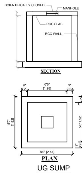
PLAN UG SUMP
