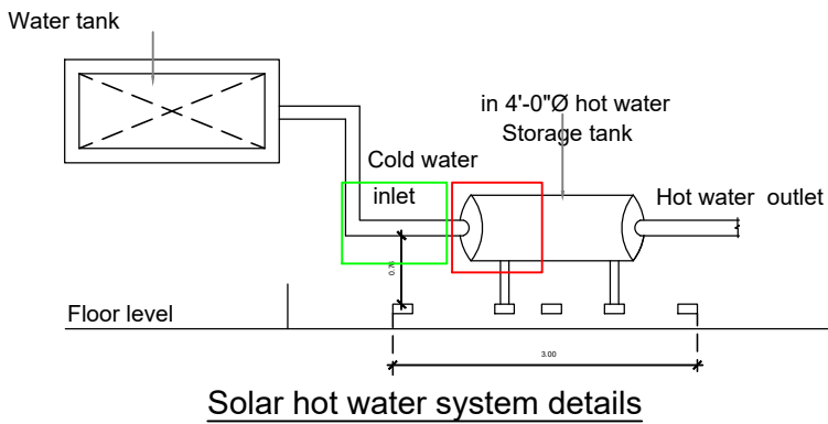
Solar hot water system details
