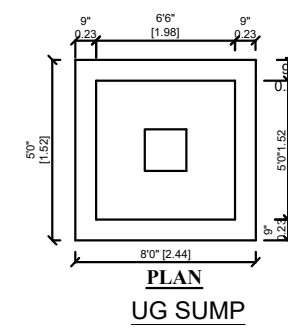
PLAN UG SUMP
