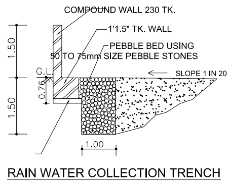
RAIN WATER COLLECTION TRENCH
