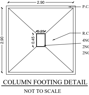
FOUNDATION DETAIL NOT TO SCALE
