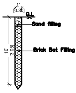
Percolation Pit Detail (Scale : Nts)
