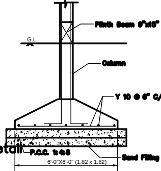
Footing Section (Scale : Nts)
