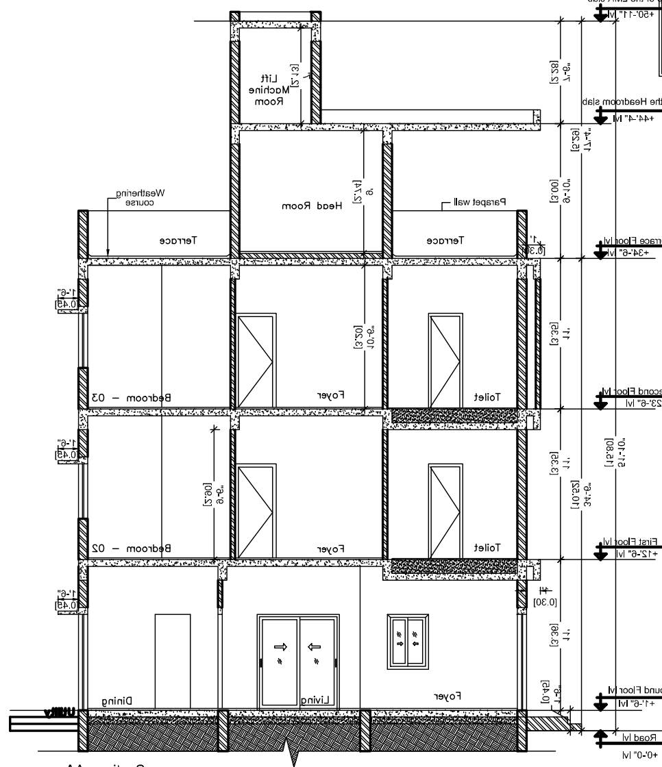
SECTION
