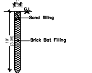
Percolation Pit Detail (Scale : Nts)
