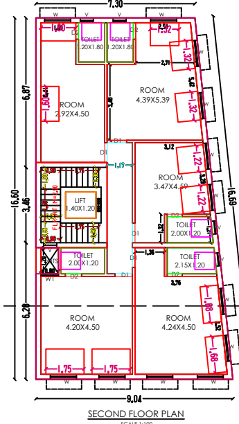
SECOND FLOOR PLAN SCALE 1:100
