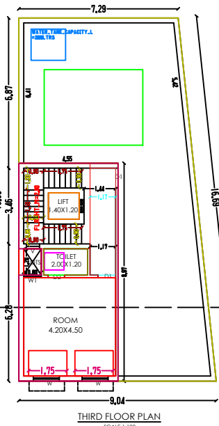
THIRD FLOOR PLAN SCALE 1:100
