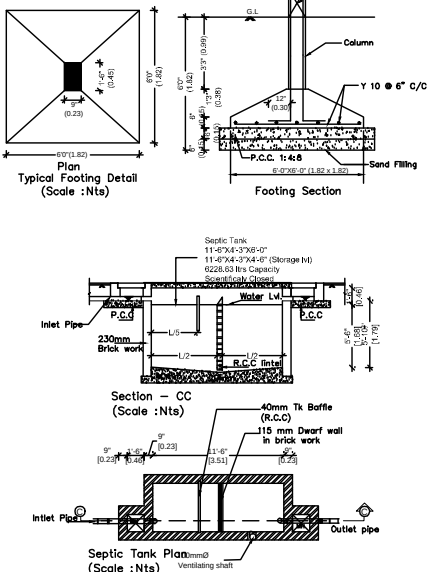
Septic Tank Plan (Scale : Nts)
