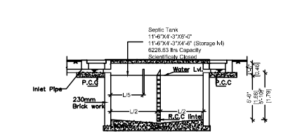
Typical Footing Detail (Scale : Nts)
