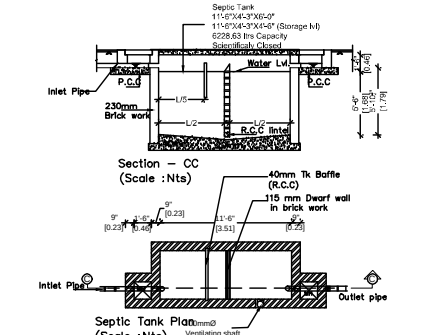
Septic Tank Plan (Scale : Nts)
