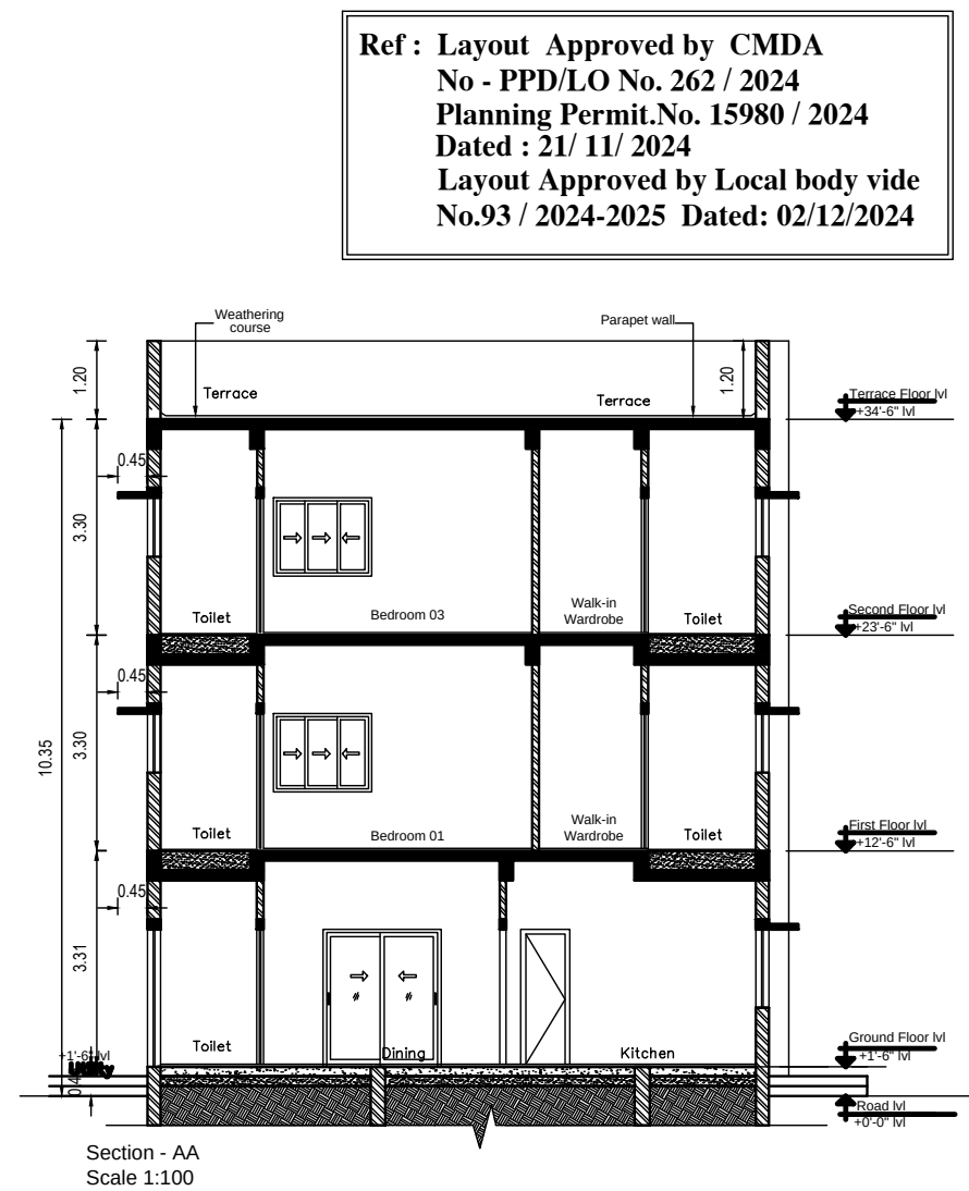
SECTION
