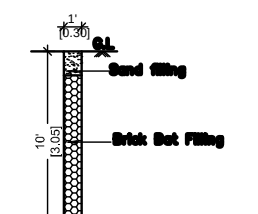
Percolation Pit Detail (Scale : Nts)
