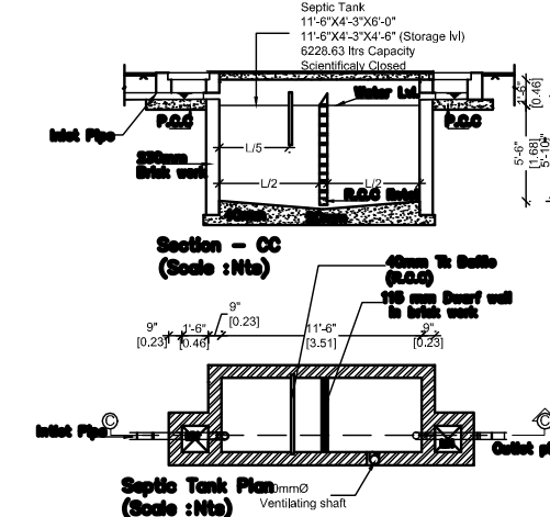
Septic Tank Plan (Scale : Nts)
