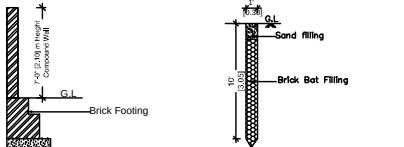
Percolation Pit Detail (Scale : Nts)
