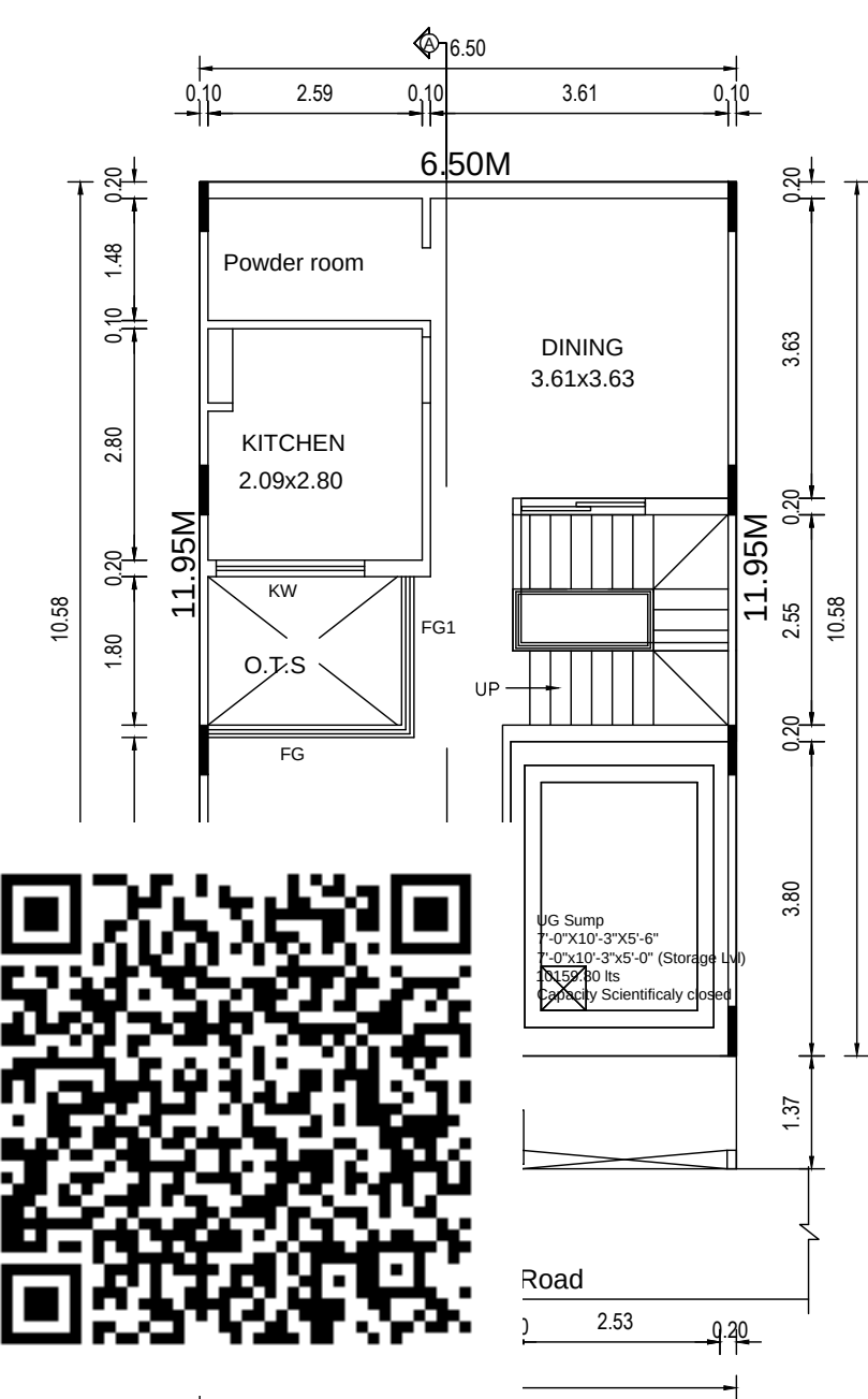
SITE CUM GROUND FLOOR PLAN
